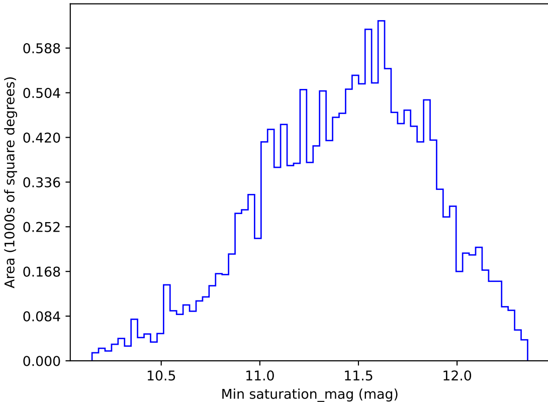
smc_lmc_v3.3_10yrs WFD u band: Min saturation_mag
