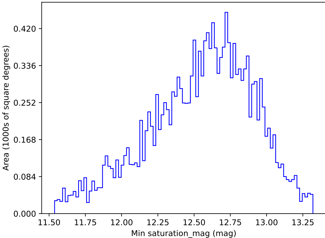
smc_lmc_v3.3_10yrs WFD r band: Min saturation_mag
