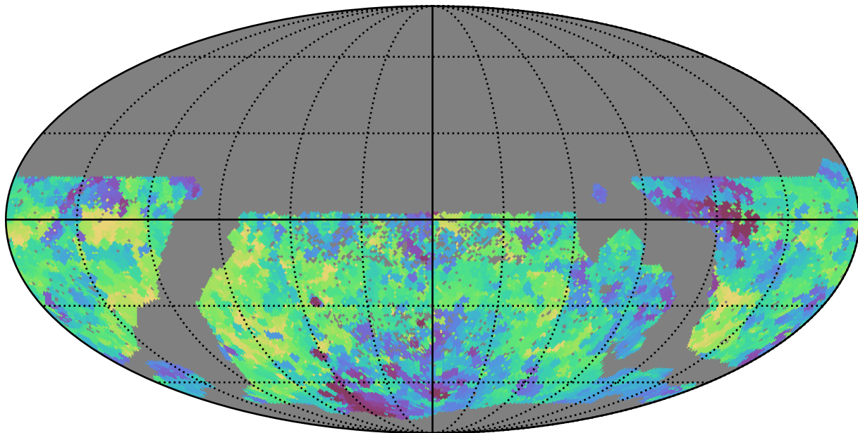
smc_lmc_v3.3_10yrs WFD g band: Min saturation_mag
