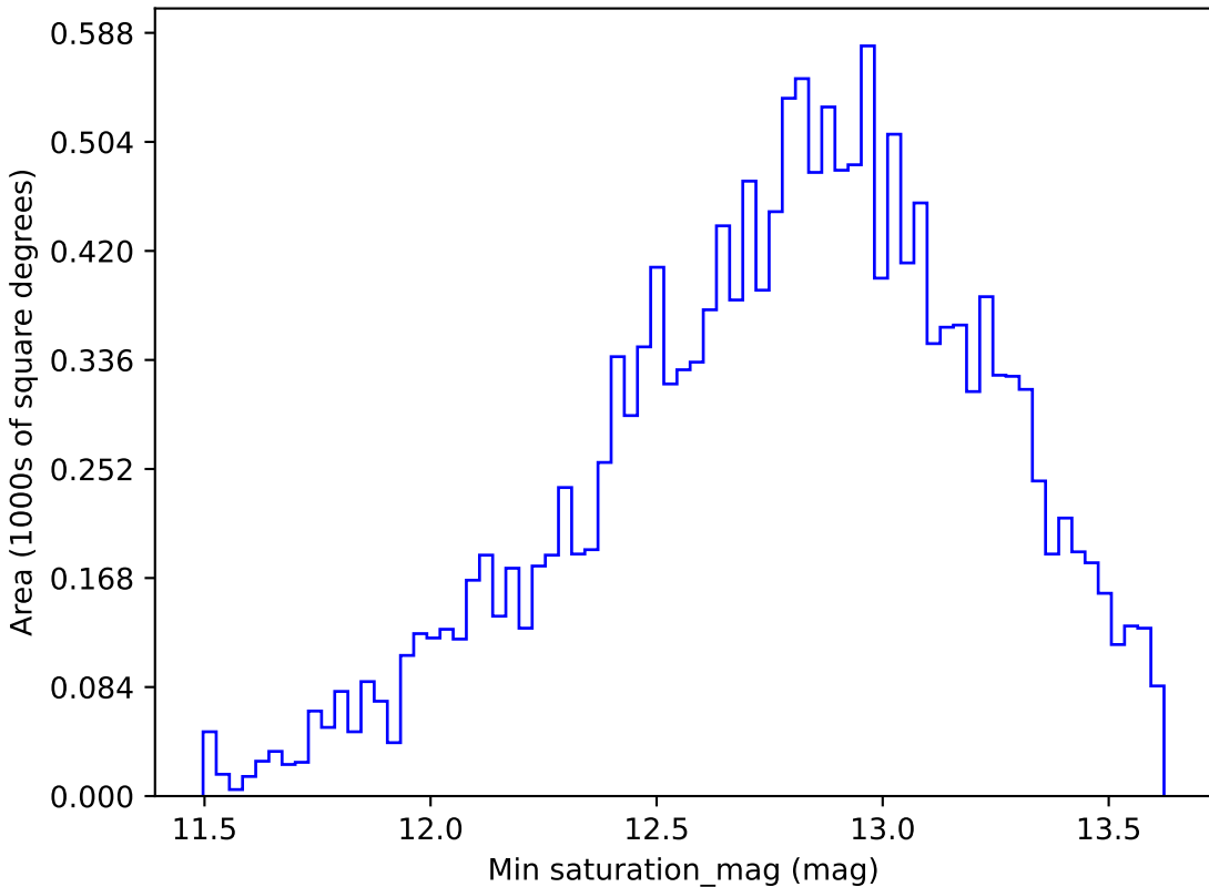
smc_lmc_v3.3_10yrs WFD g band: Min saturation_mag
