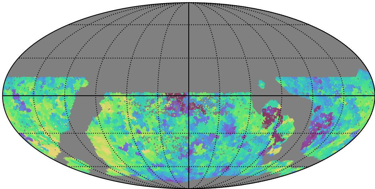
smc_lmc_v3.3_10yrs WFD all bands: Min saturation_mag
