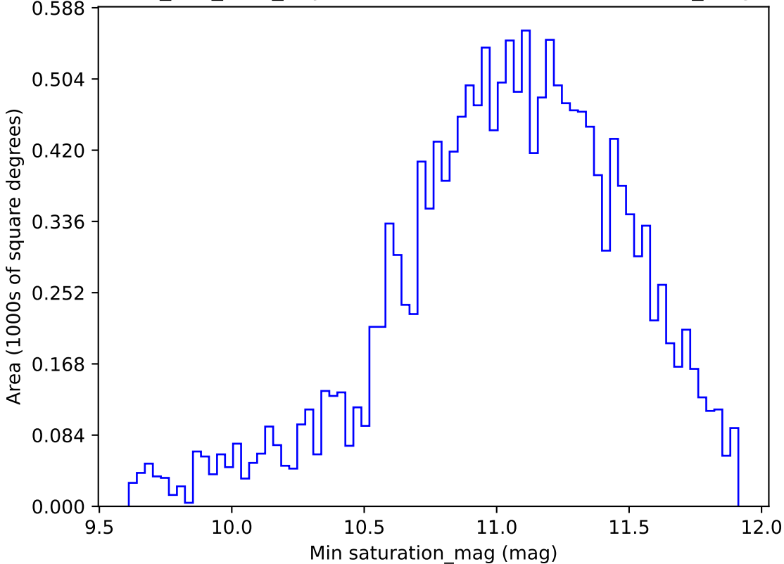
smc_lmc_v3.3_10yrs WFD all bands: Min saturation_mag
