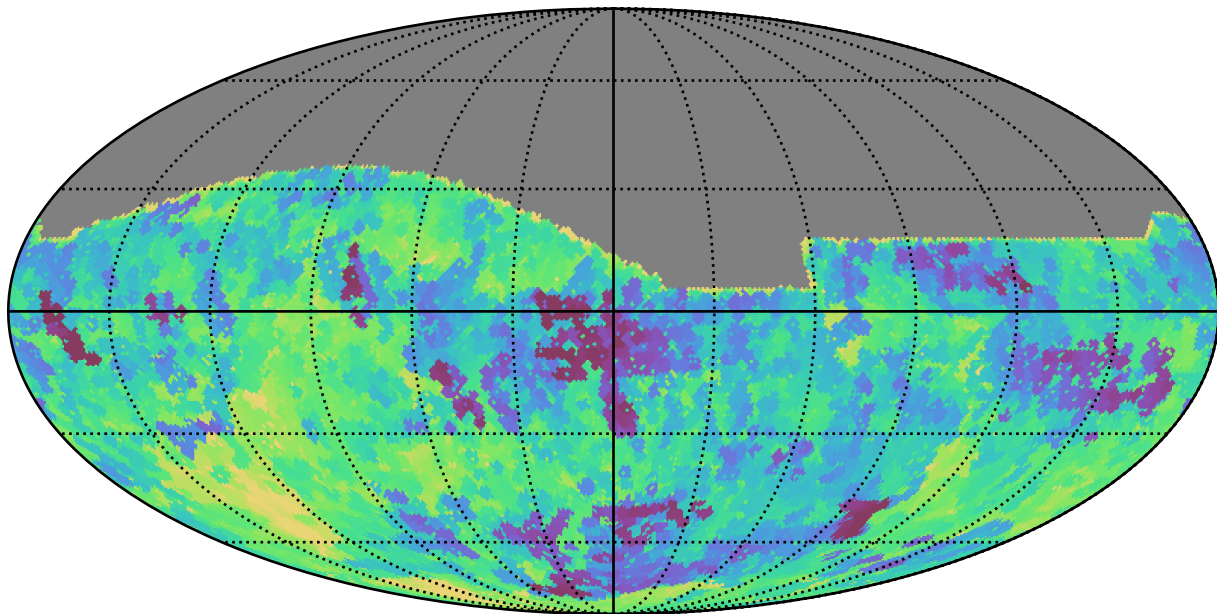
smc_lmc_v3.3_10yrs All sky z band: Min saturation_mag
