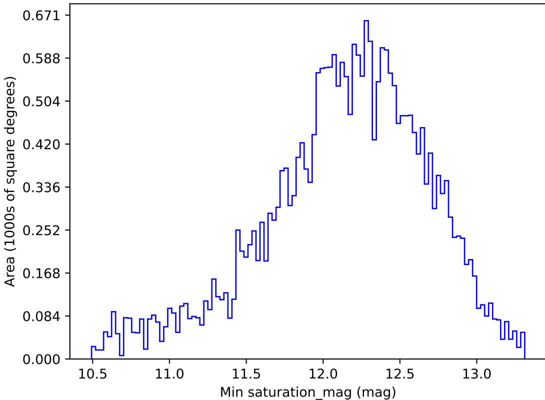
smc_lmc_v3.3_10yrs All sky z band: Min saturation_mag
