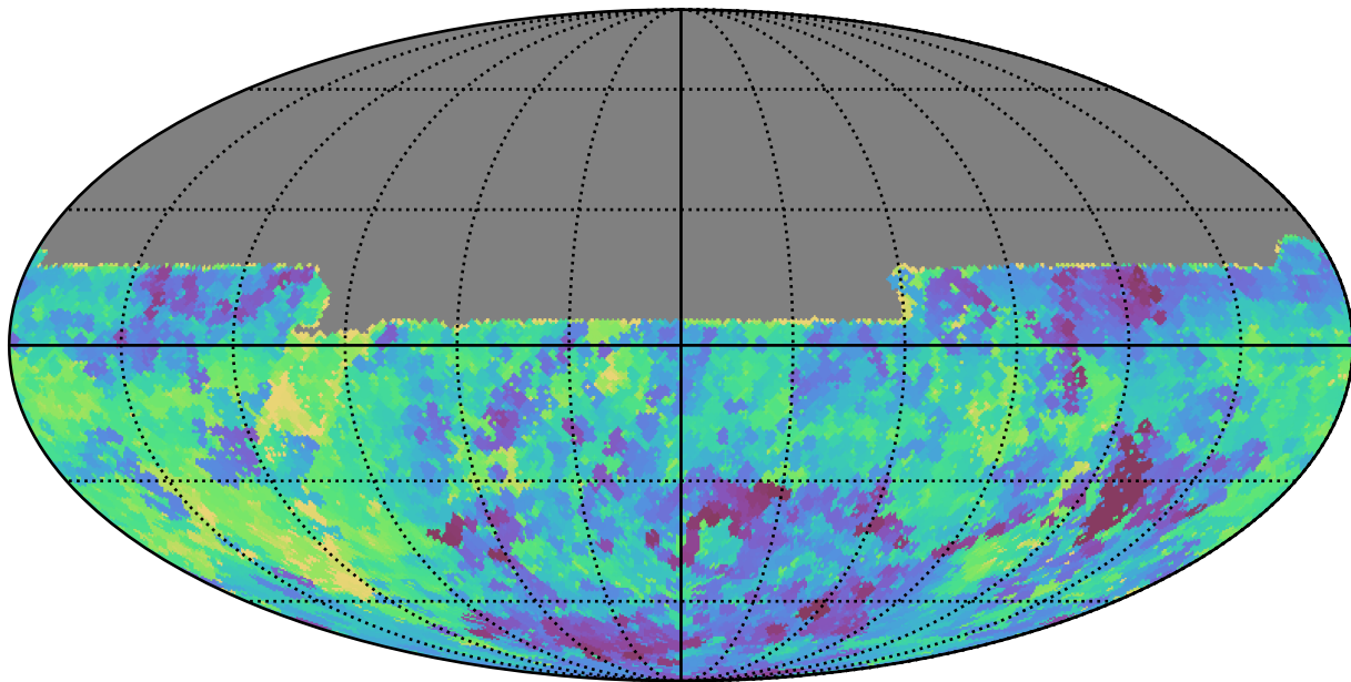
smc_lmc_v3.3_10yrs All sky u band: Min saturation_mag
