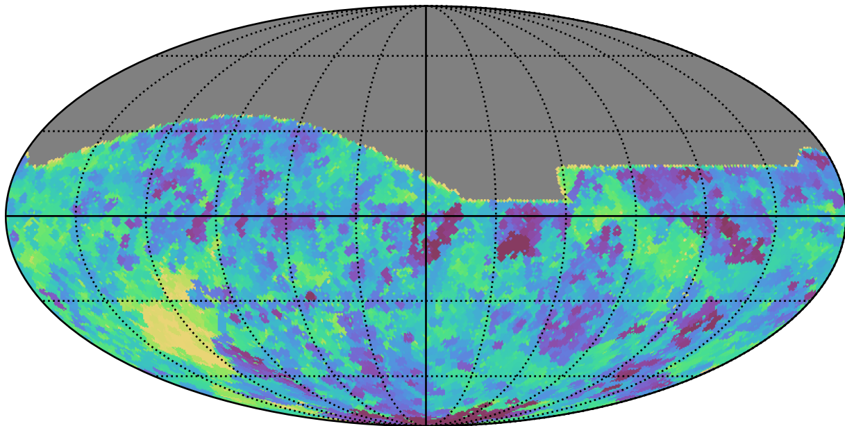
smc_lmc_v3.3_10yrs All sky r band: Min saturation_mag
