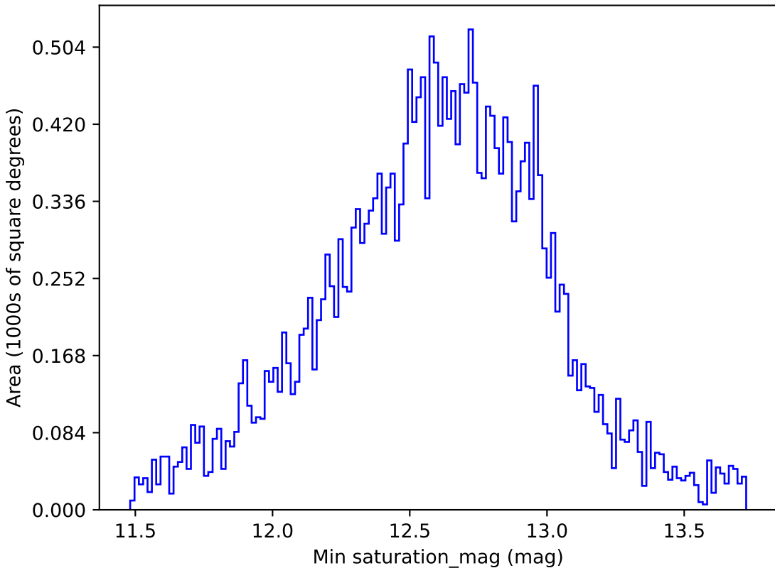
smc_lmc_v3.3_10yrs All sky r band: Min saturation_mag
