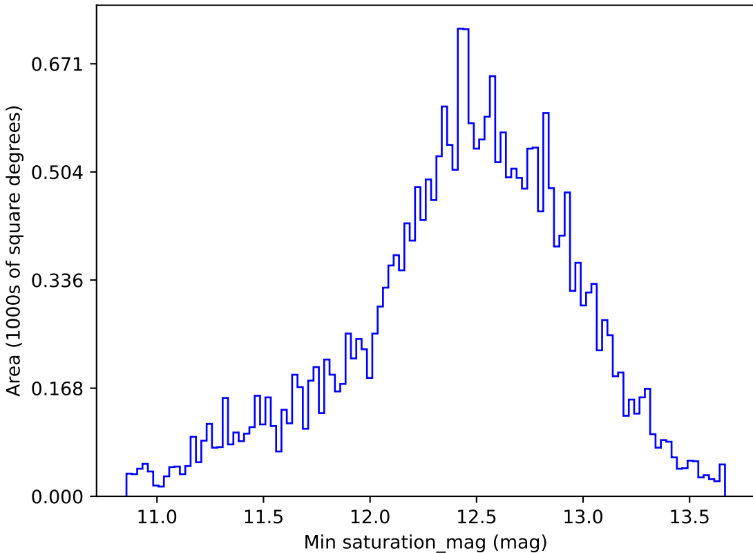
smc_lmc_v3.3_10yrs All sky i band: Min saturation_mag
