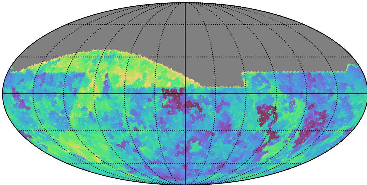
smc_lmc_v3.3_10yrs All sky all bands: Min saturation_mag
