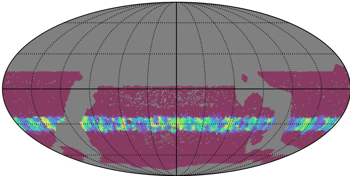
smc_lmc_v3.3_10yrs WFD z band: Min normairmass
