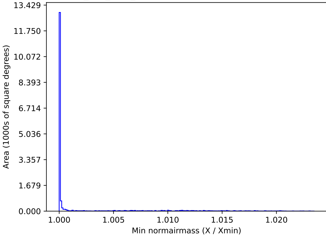
smc_lmc_v3.3_10yrs WFD z band: Min normairmass
