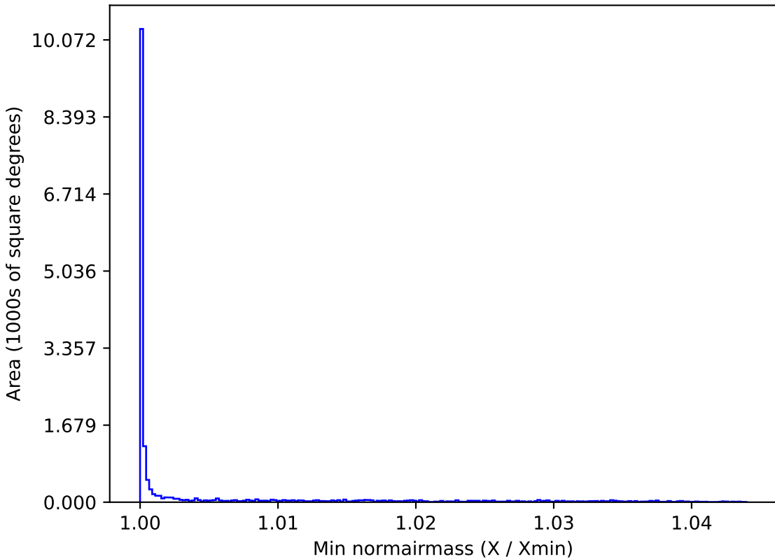
smc_lmc_v3.3_10yrs WFD u band: Min normairmass
