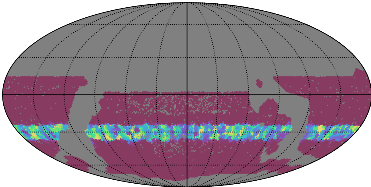
smc_lmc_v3.3_10yrs WFD r band: Min normairmass
