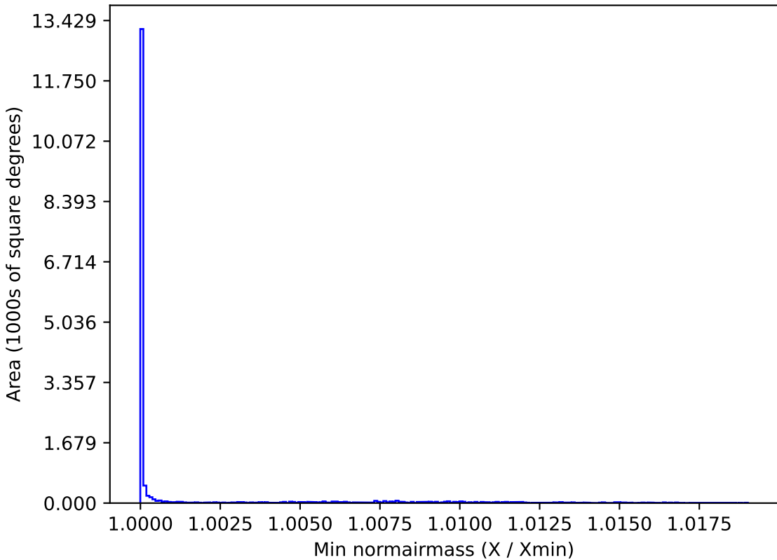
smc_lmc_v3.3_10yrs WFD r band: Min normairmass
