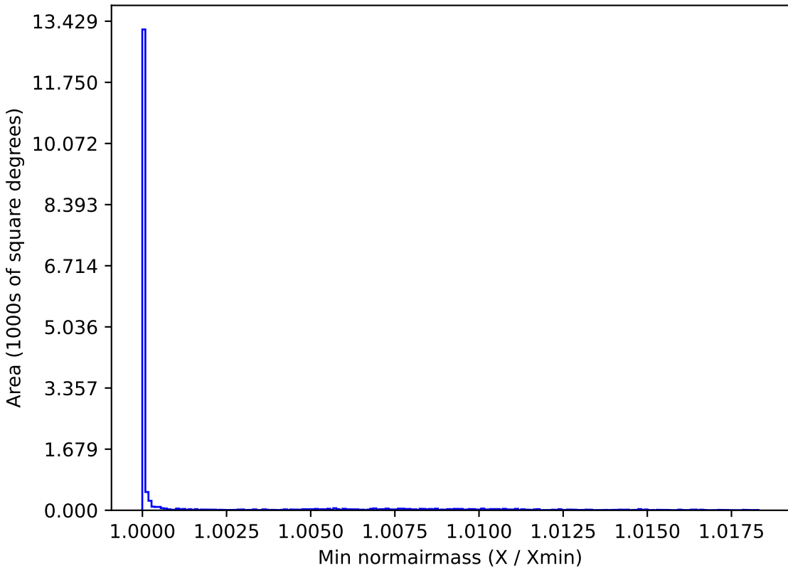
smc_lmc_v3.3_10yrs WFD i band: Min normairmass
