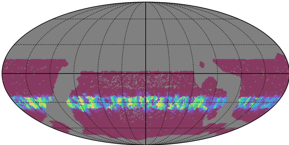
smc_lmc_v3.3_10yrs WFD g band: Min normairmass
