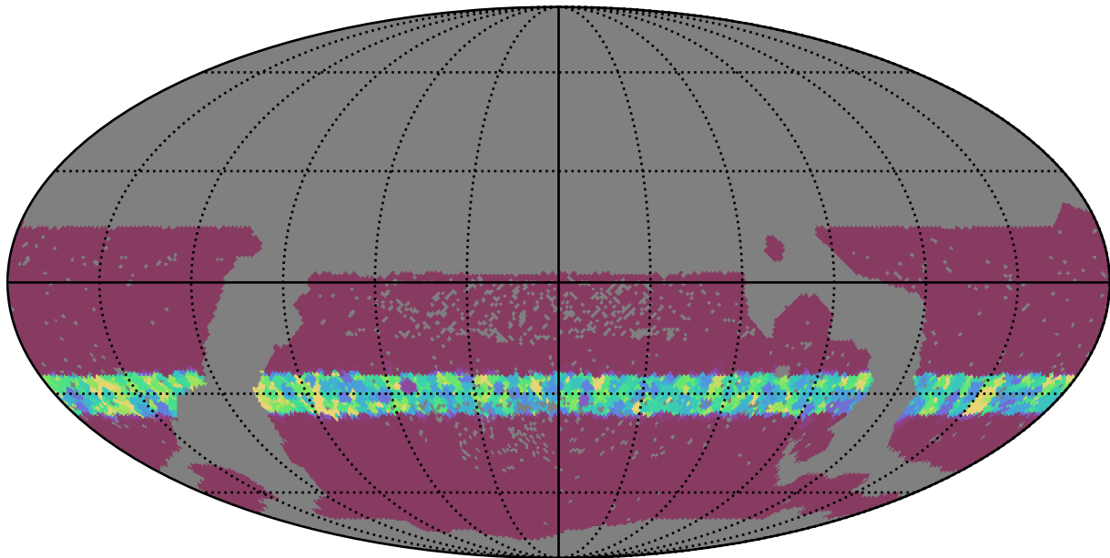
smc_lmc_v3.3_10yrs WFD all bands: Min normairmass
