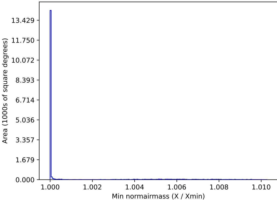
smc_lmc_v3.3_10yrs WFD all bands: Min normairmass
