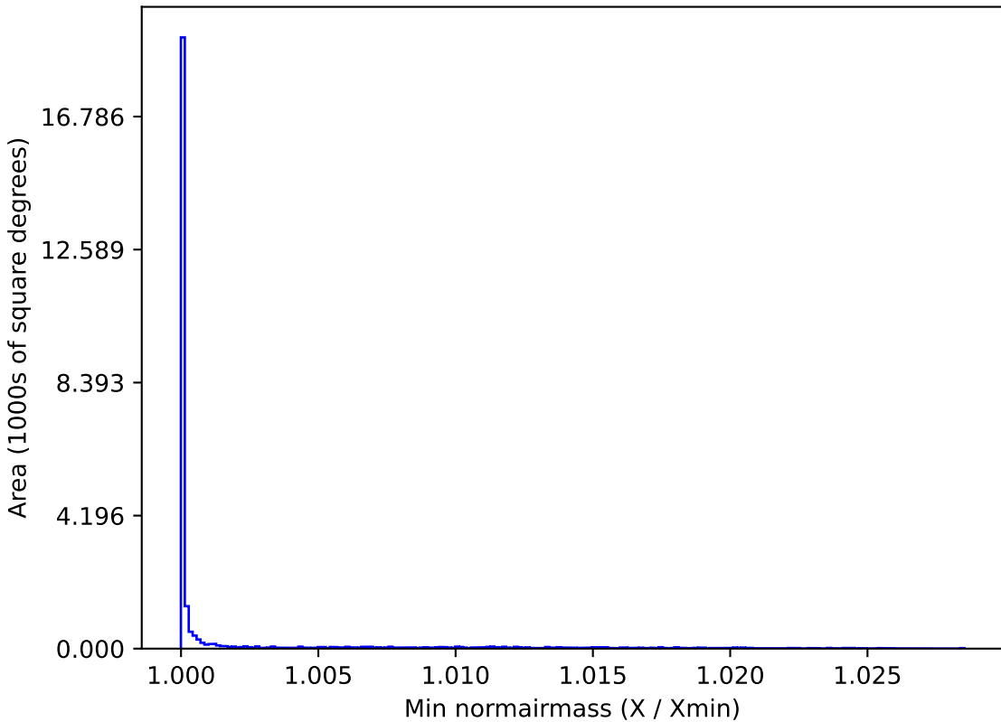
smc_lmc_v3.3_10yrs All sky z band: Min normairmass
