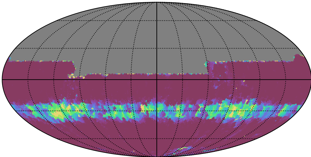
smc_lmc_v3.3_10yrs All sky u band: Min normairmass
