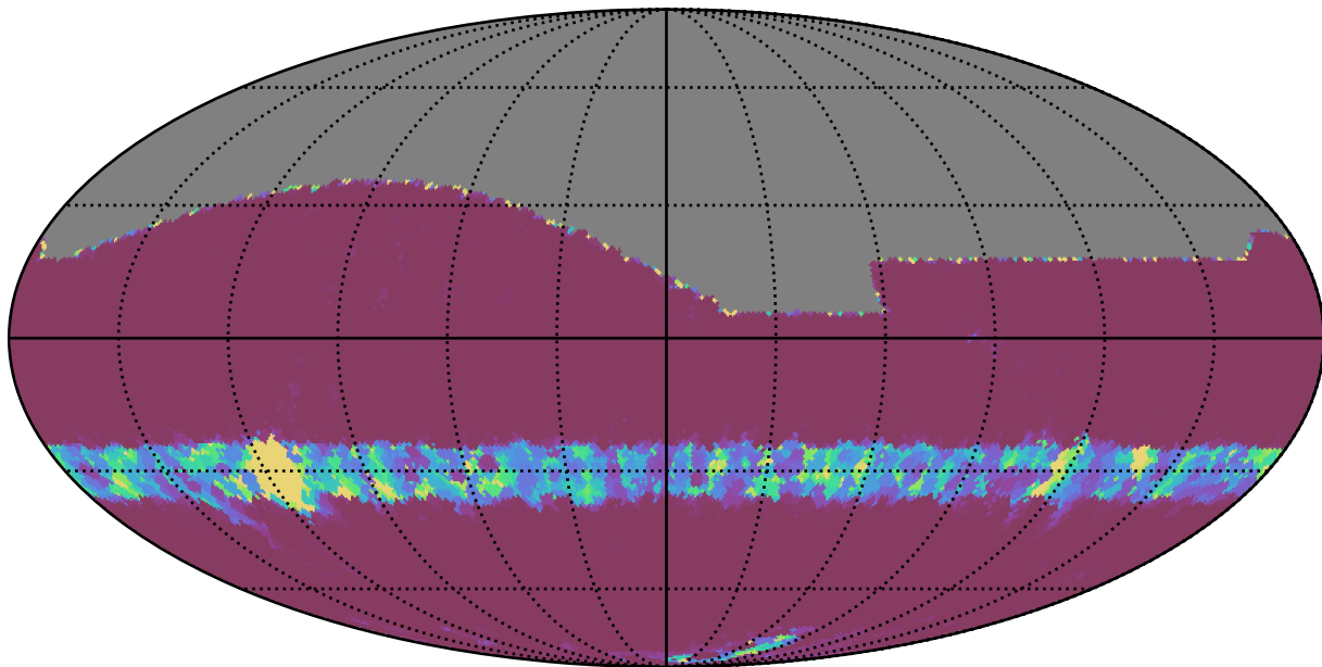
smc_lmc_v3.3_10yrs All sky r band: Min normairmass
