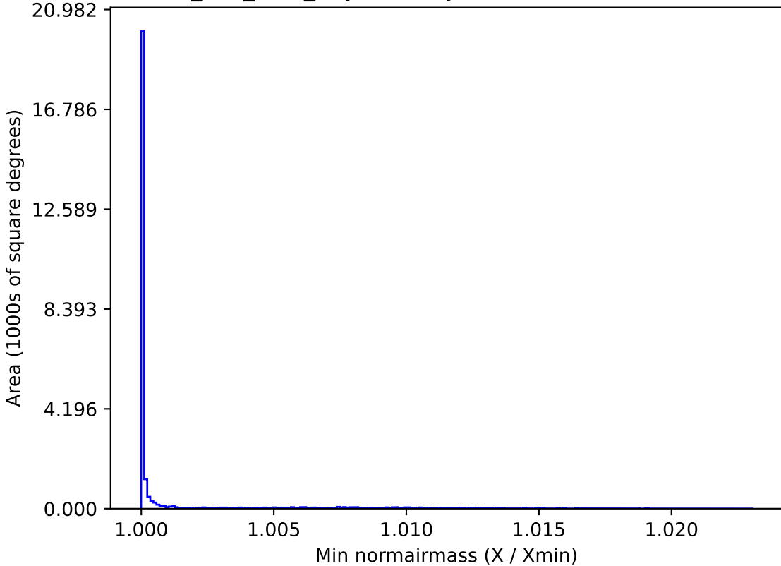
smc_lmc_v3.3_10yrs All sky r band: Min normairmass
