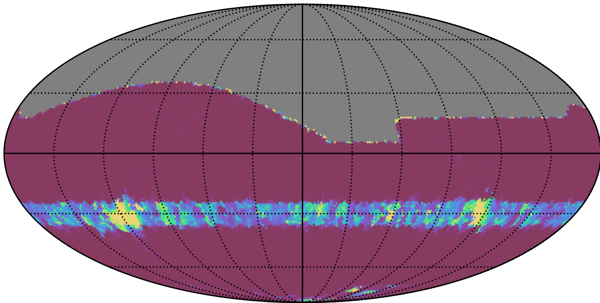
smc_lmc_v3.3_10yrs All sky i band: Min normairmass
