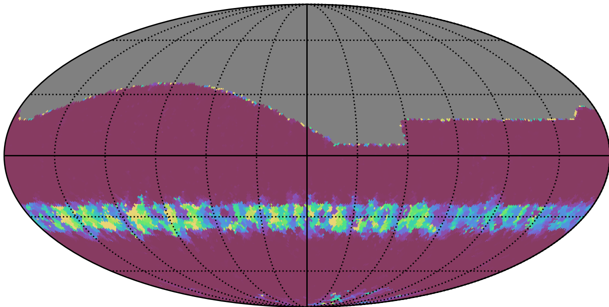
smc_lmc_v3.3_10yrs All sky g band: Min normairmass
