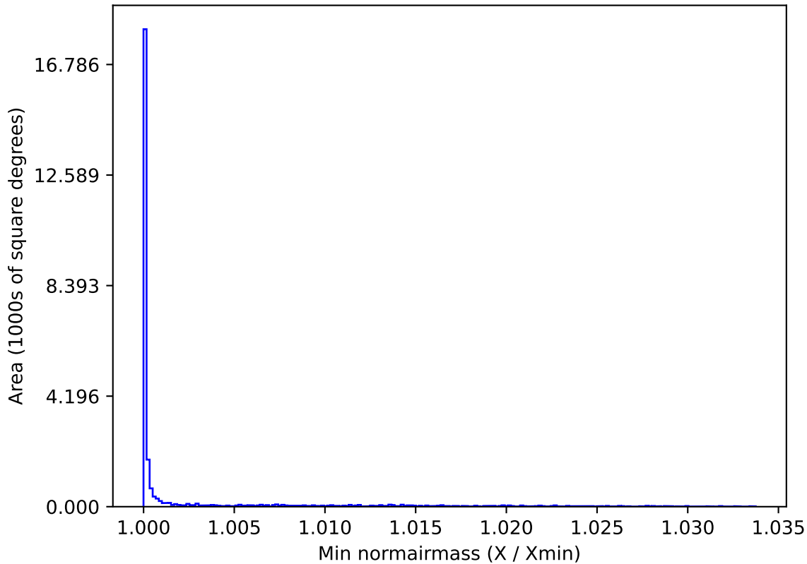
smc_lmc_v3.3_10yrs All sky g band: Min normairmass
