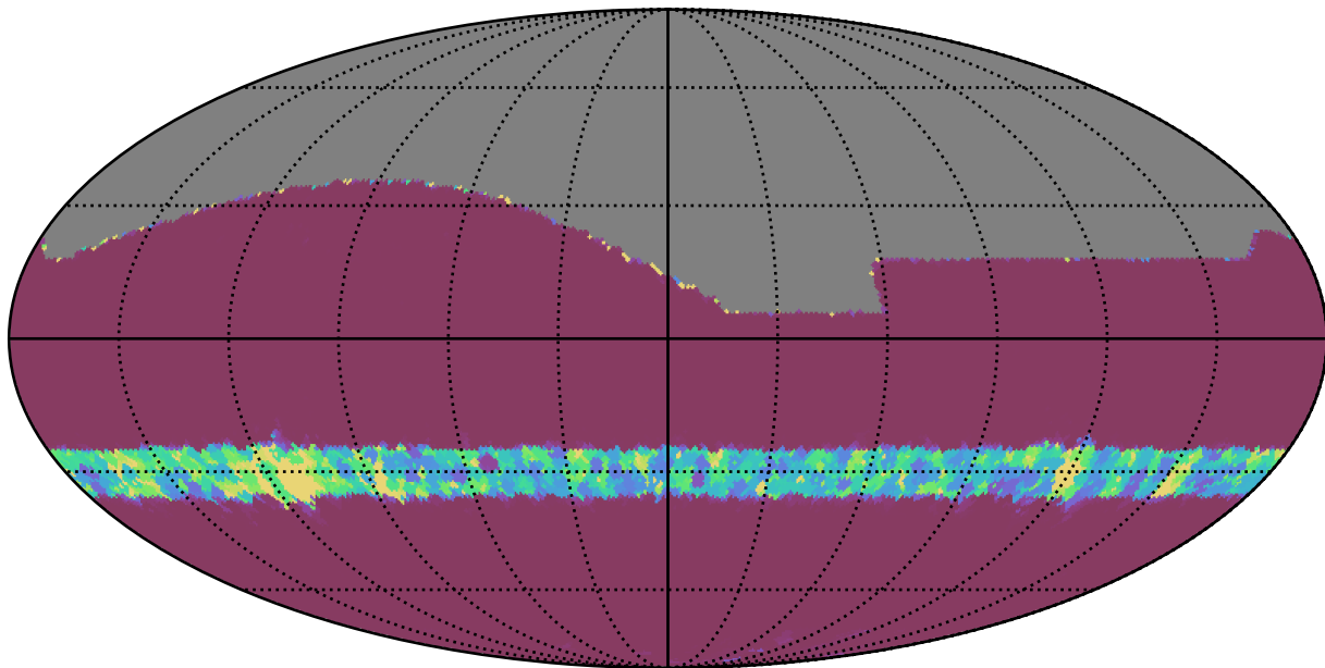
smc_lmc_v3.3_10yrs All sky all bands: Min normairmass
