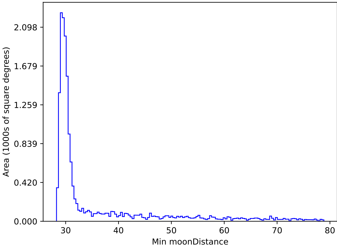
smc_lmc_v3.3_10yrs WFD z band: Min moonDistance
