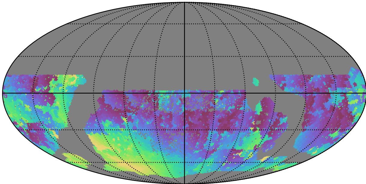
smc_lmc_v3.3_10yrs WFD u band: Min moonDistance
