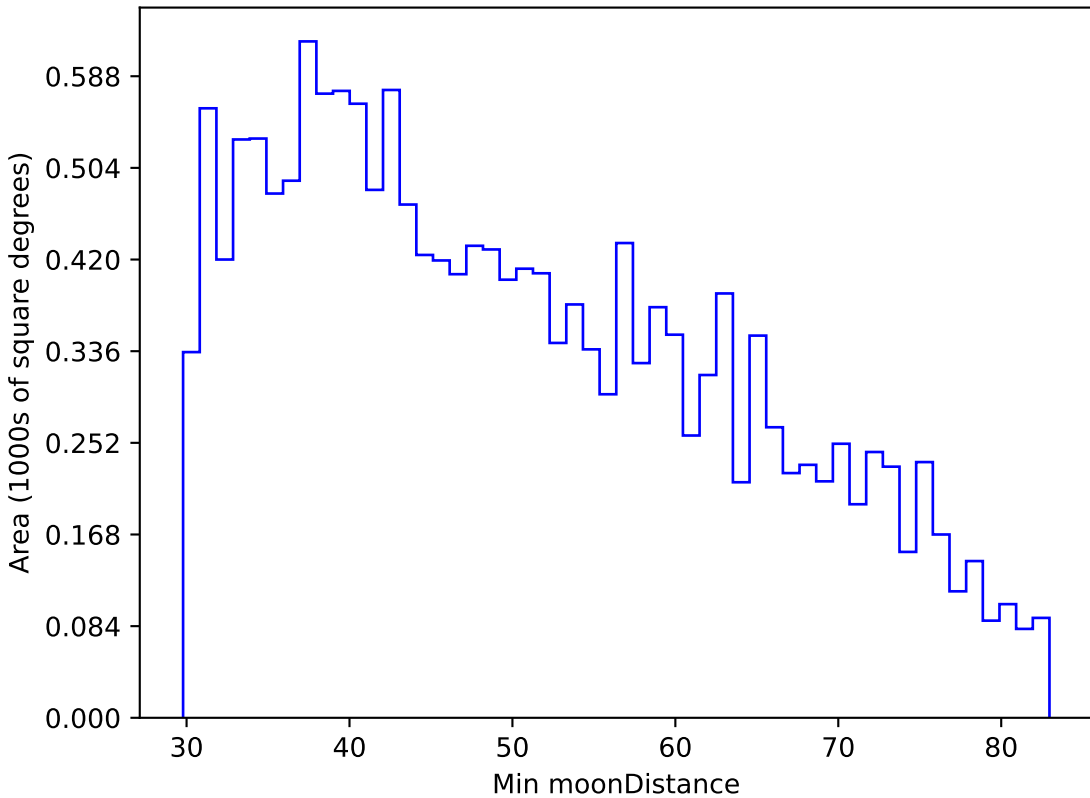
smc_lmc_v3.3_10yrs WFD u band: Min moonDistance
