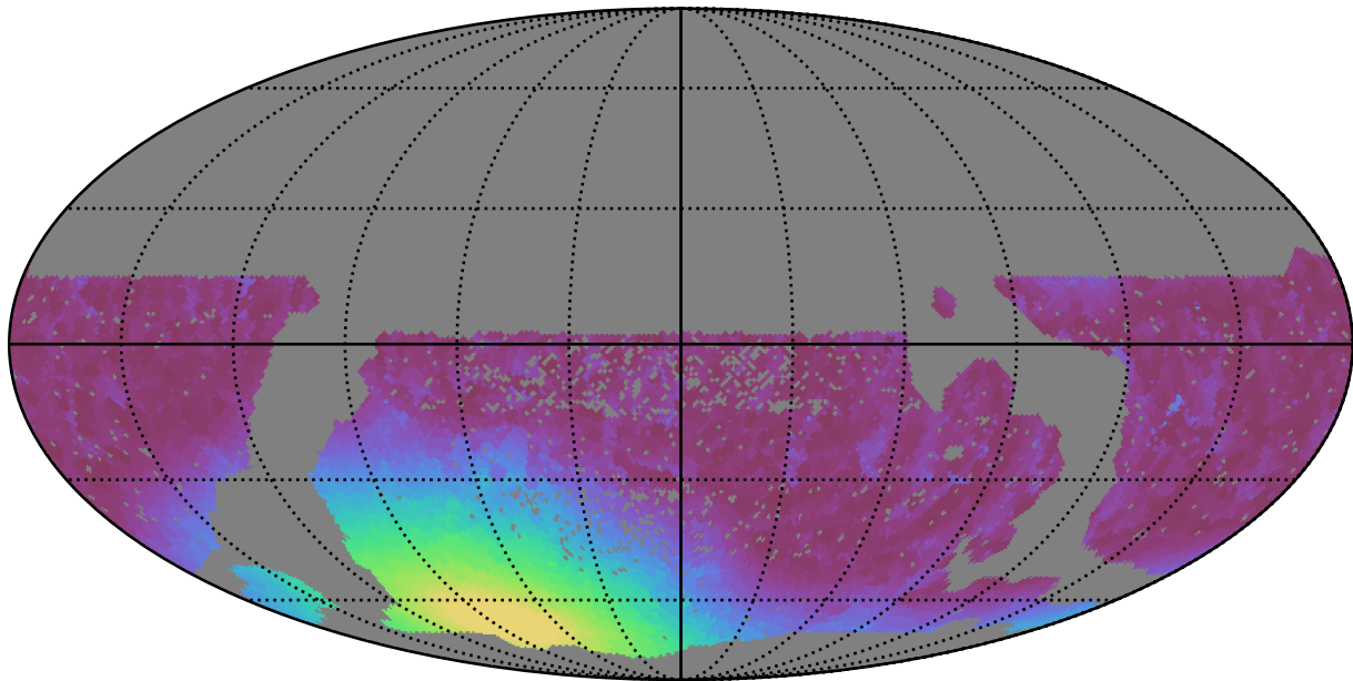
smc_lmc_v3.3_10yrs WFD r band: Min moonDistance
