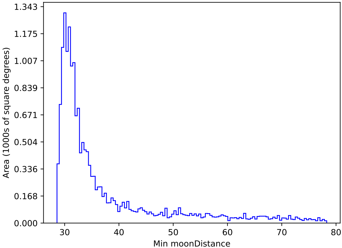
smc_lmc_v3.3_10yrs WFD r band: Min moonDistance
