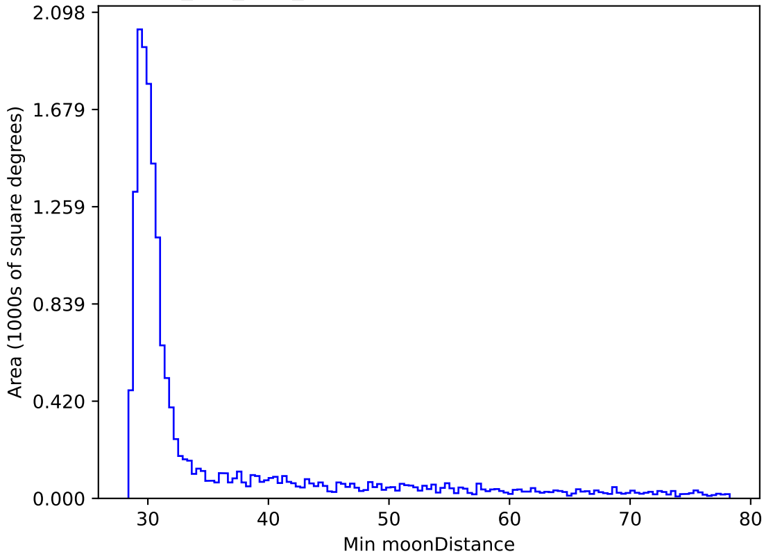
smc_lmc_v3.3_10yrs WFD i band: Min moonDistance
