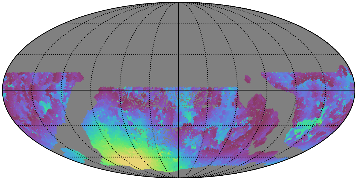
smc_lmc_v3.3_10yrs WFD g band: Min moonDistance
