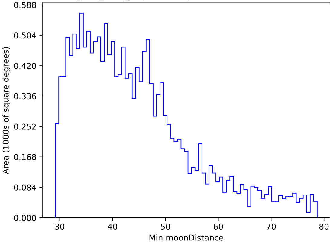
smc_lmc_v3.3_10yrs WFD g band: Min moonDistance
