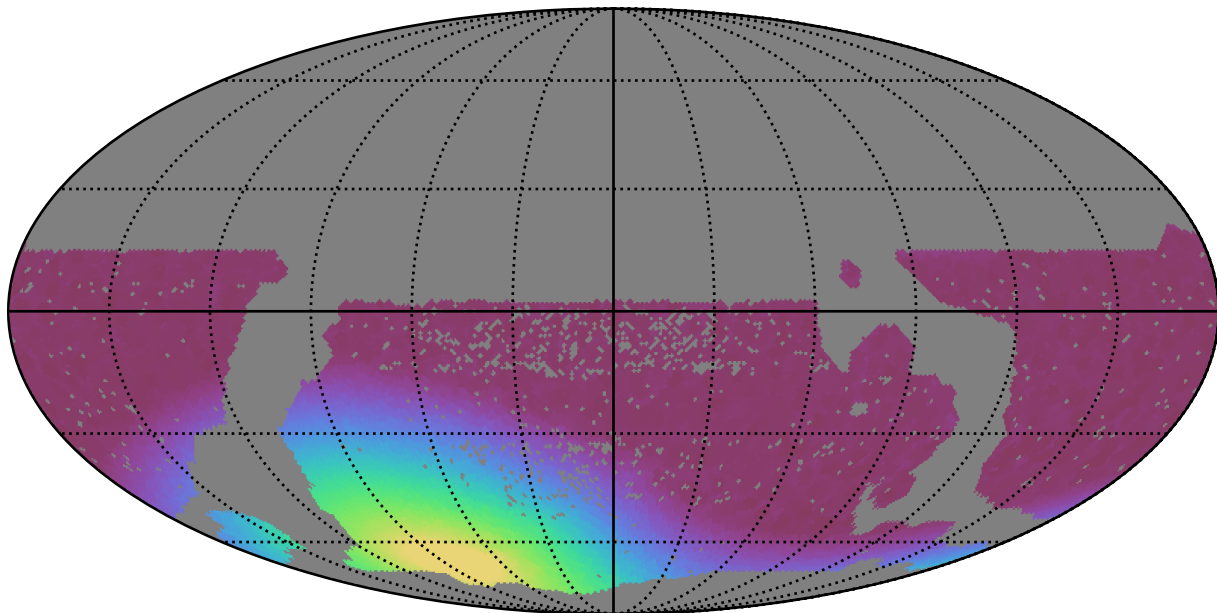
smc_lmc_v3.3_10yrs WFD all bands: Min moonDistance
