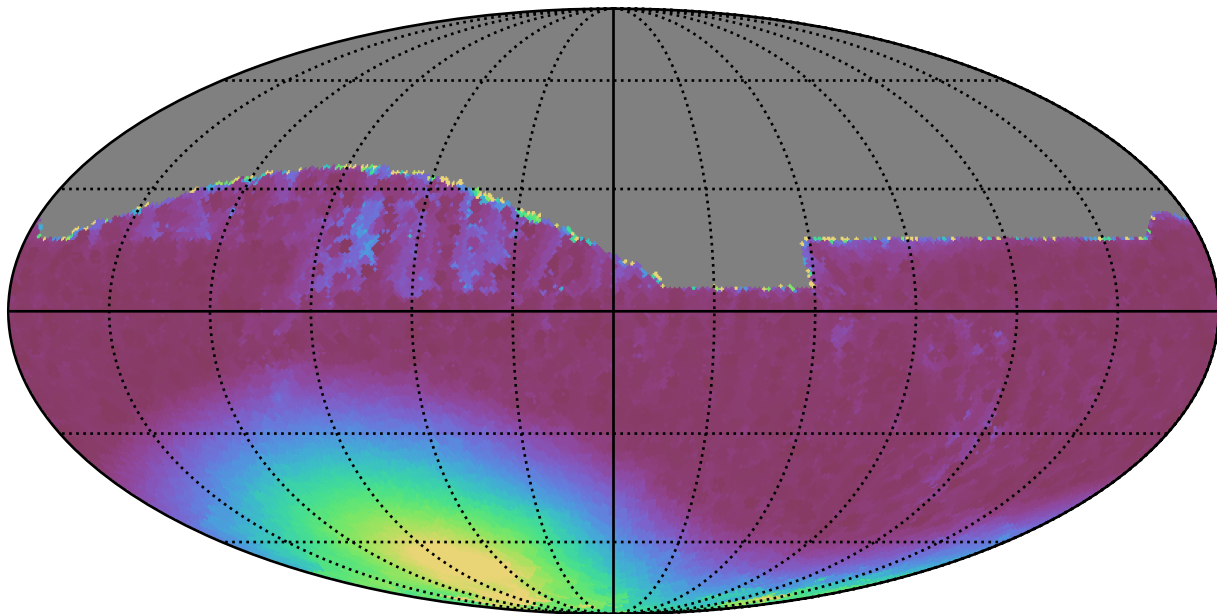
smc_lmc_v3.3_10yrs All sky z band: Min moonDistance
