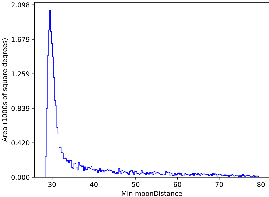
smc_lmc_v3.3_10yrs All sky z band: Min moonDistance
