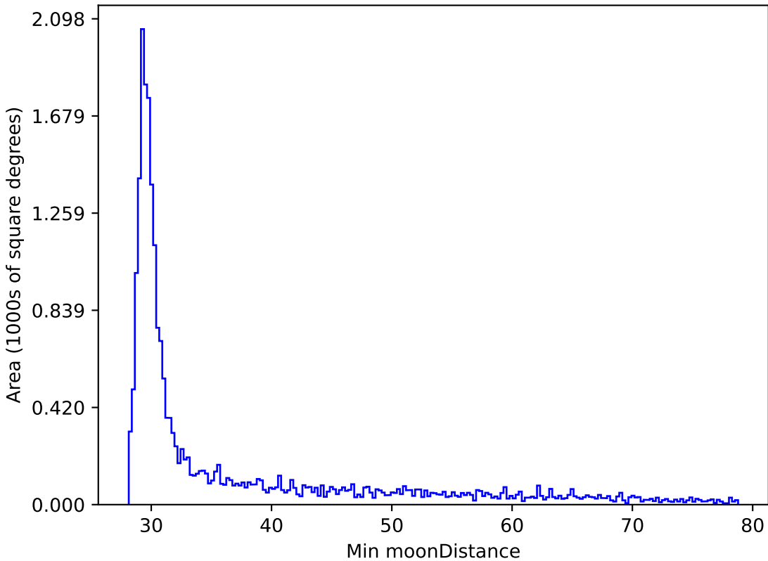
smc_lmc_v3.3_10yrs All sky y band: Min moonDistance
