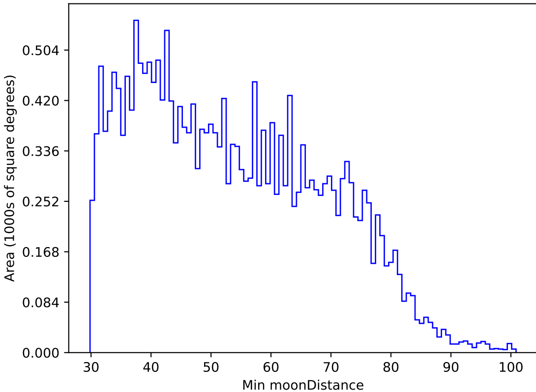
smc_lmc_v3.3_10yrs All sky u band: Min moonDistance
