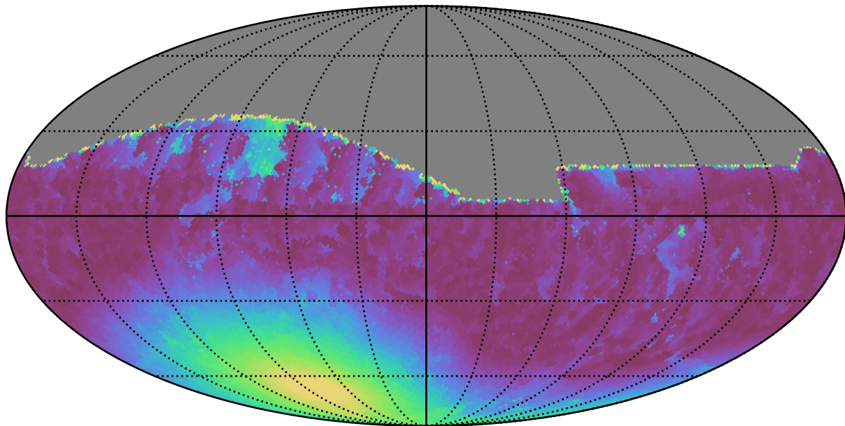
smc_lmc_v3.3_10yrs All sky r band: Min moonDistance
