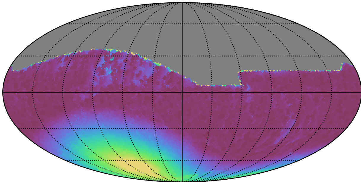
smc_lmc_v3.3_10yrs All sky i band: Min moonDistance
