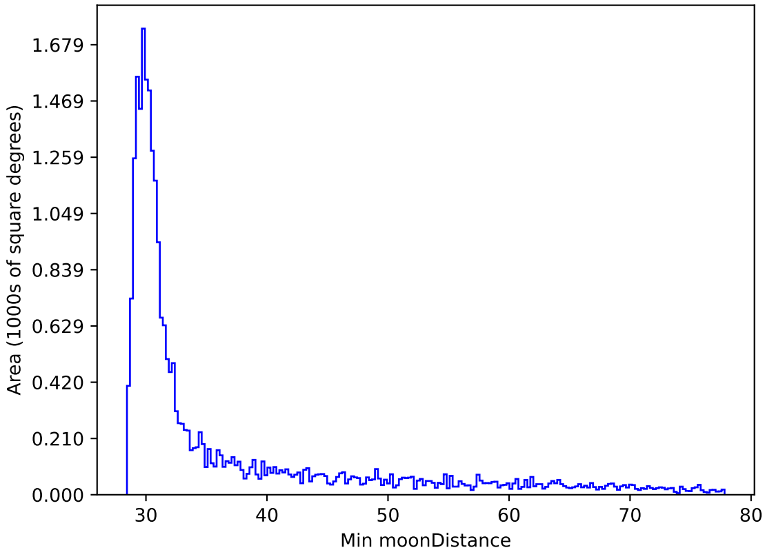
smc_lmc_v3.3_10yrs All sky i band: Min moonDistance
