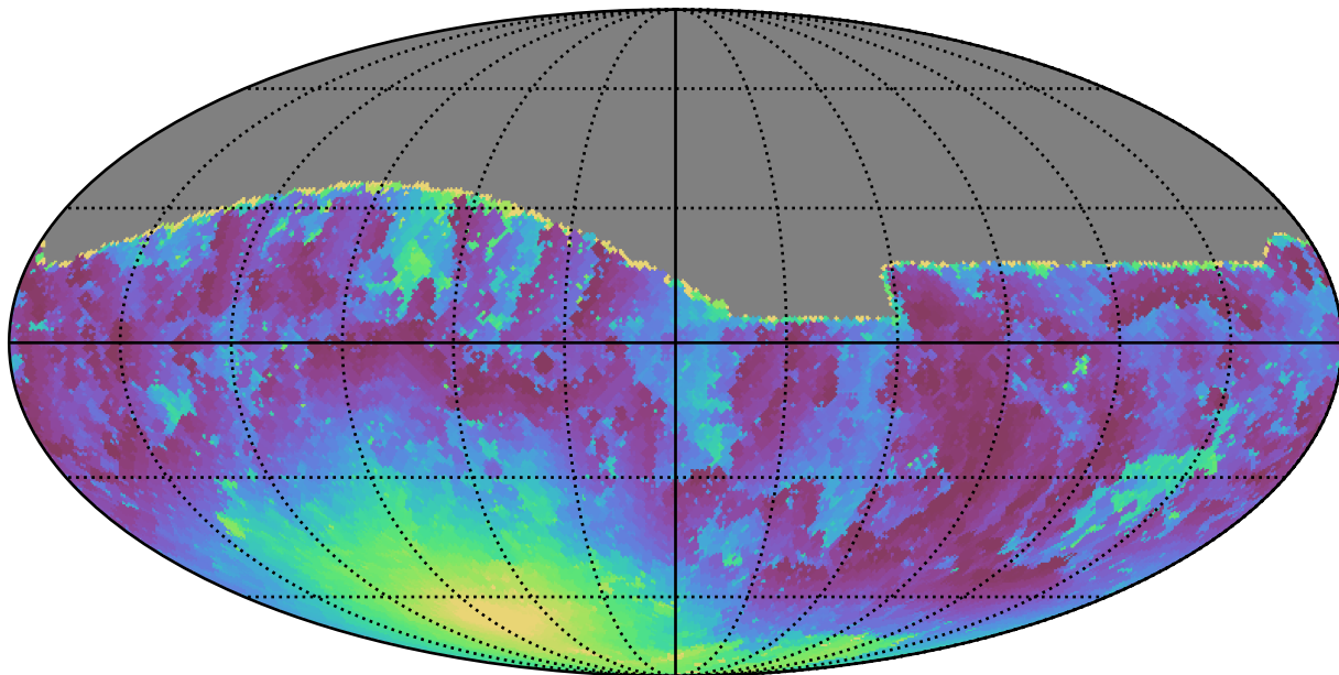
smc_lmc_v3.3_10yrs All sky g band: Min moonDistance
