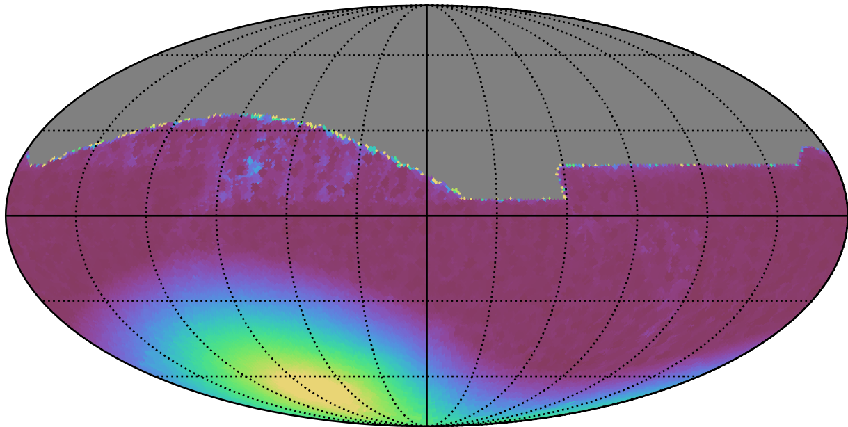
smc_lmc_v3.3_10yrs All sky all bands: Min moonDistance
