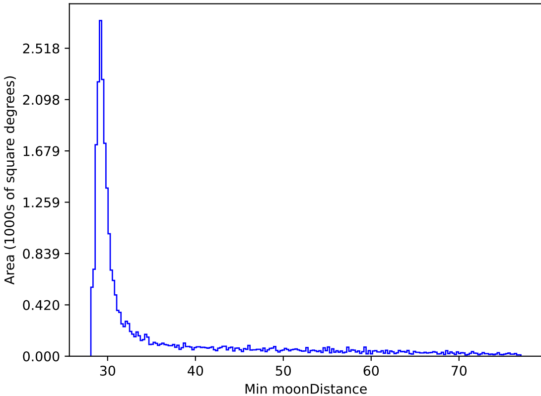
smc_lmc_v3.3_10yrs All sky all bands: Min moonDistance
