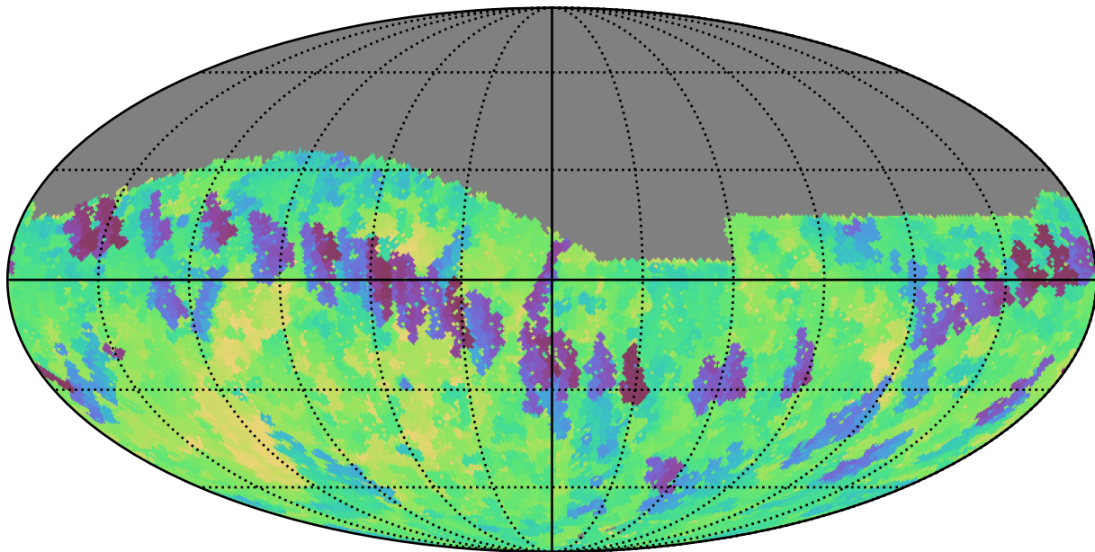
smc_lmc_v3.3_10yrs Yr 1 z band: Min fiveSigmaDepth
